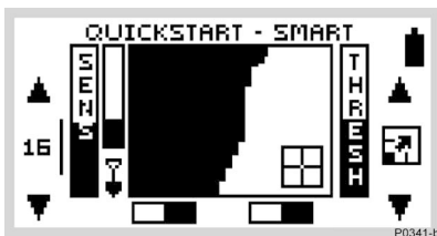
Figure 5.4 Smartfind's preset Discrim function
